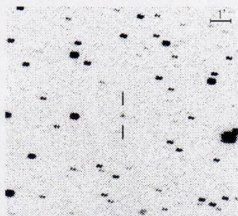
C/1997BA6 (Spacewatch) Feb. 17, 1998
