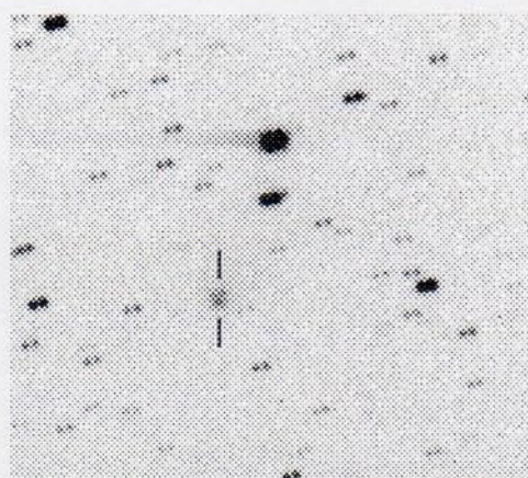
43P/Wolf-Harrington Feb. 17, 1998
